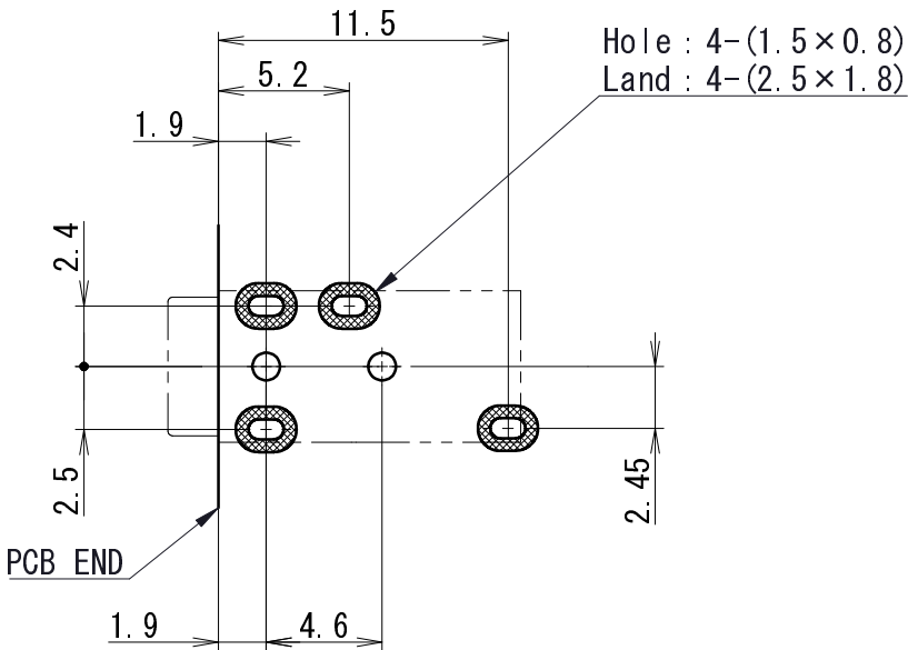
PCB Layout (DIP) (Top View)
