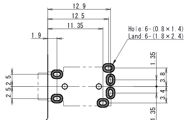
PCB Layout (DIP) (Top View)
