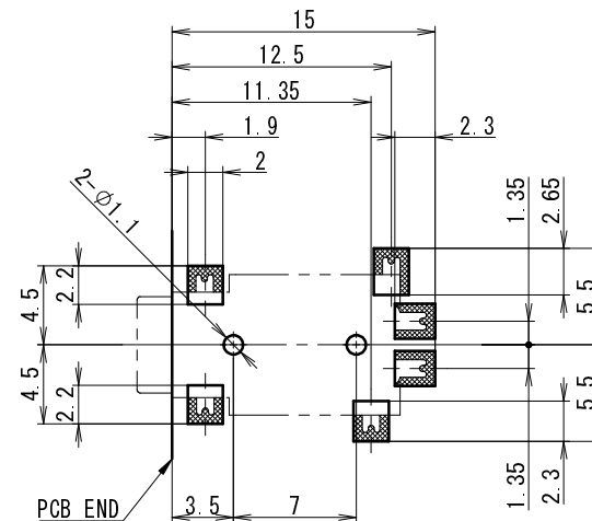
PCB Layout (SMT) (Top View)
