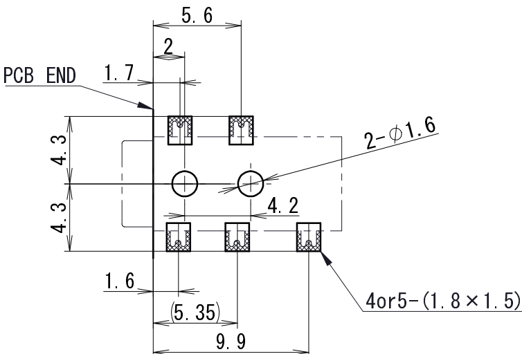
PCB Layout (SMT) (Top View)
