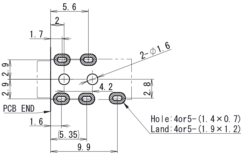
PCB Layout (DIP) (Top View)
