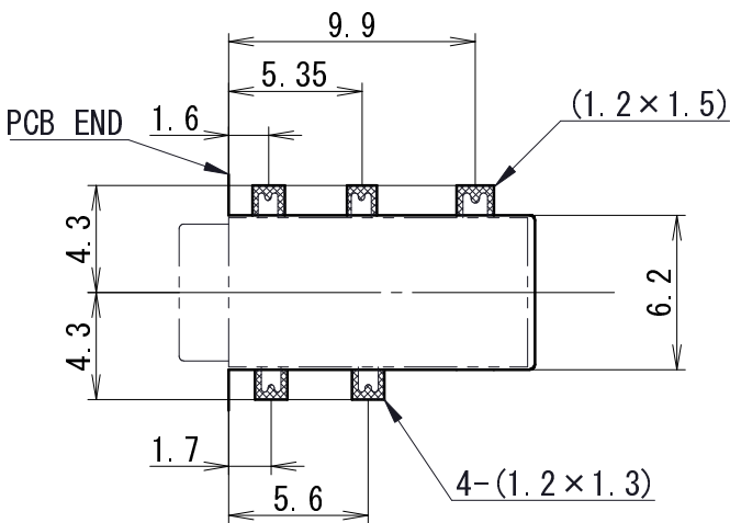
PCB Layout (MID) (Bottom View)
