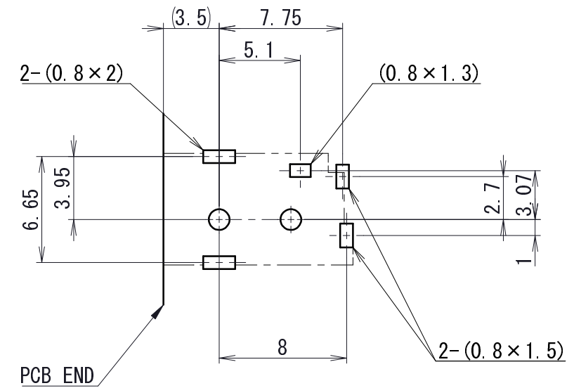
PCB Layout (DIP) (Top View)
