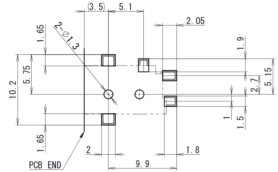
PCB Layout (SMT) (Top View)
